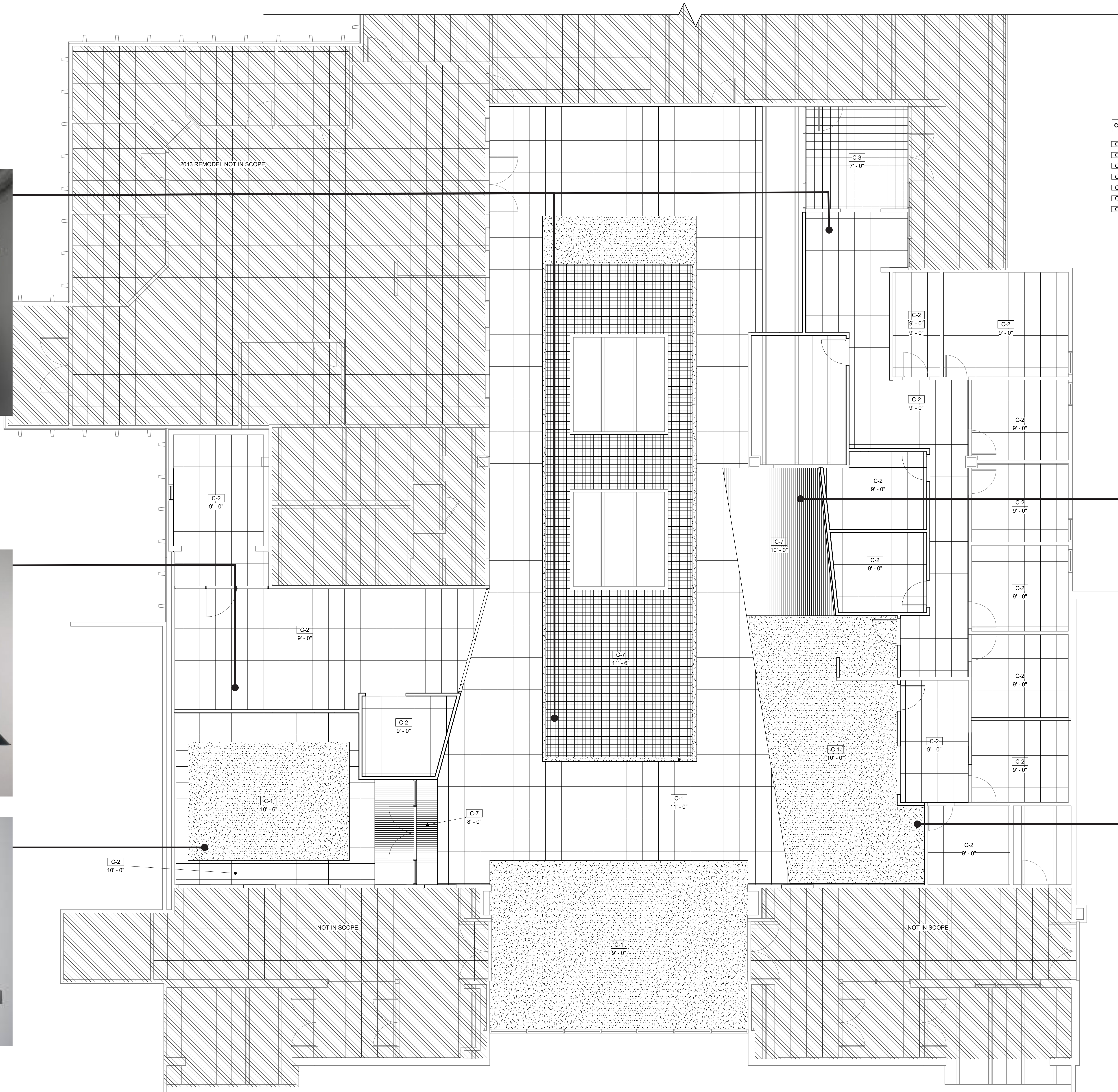
REFLECTED CEILING PLAN
