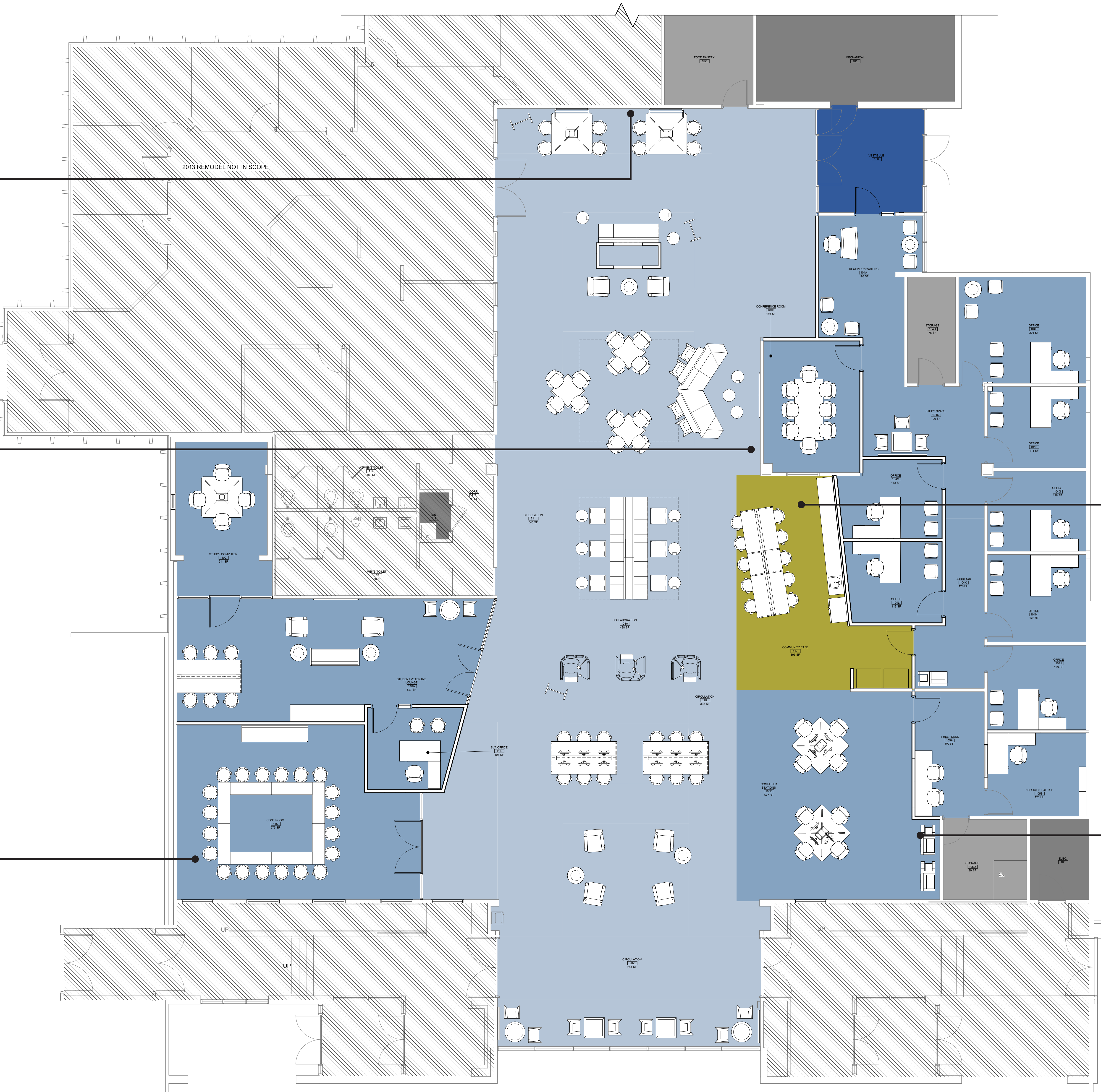
FLOOR FINISH PLAN
